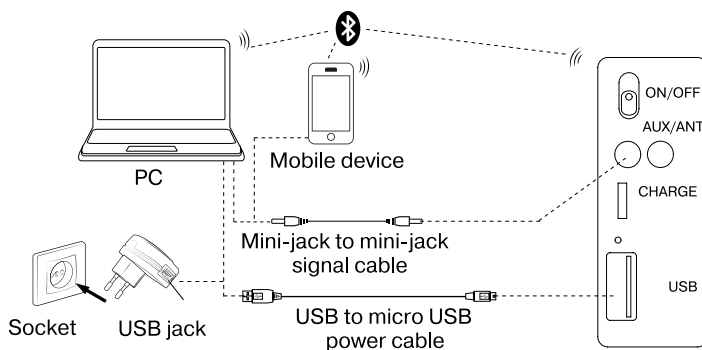
Fig. 2. Connection diagram
